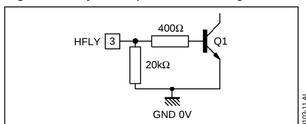
Figure 16 : Flyback Input Electrical Diagram
