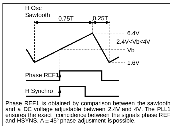
Figure 13 : PLL1 Timing Diagram
